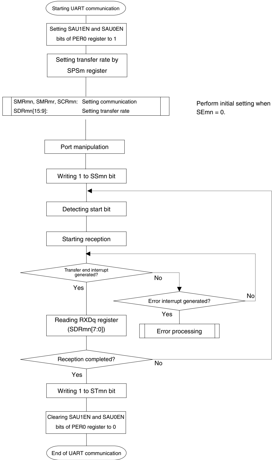
Figure 12-84. Flowchart of UART Reception
