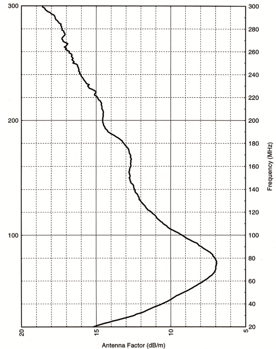
HBA-2030 Antenna Factor - 3 meter
