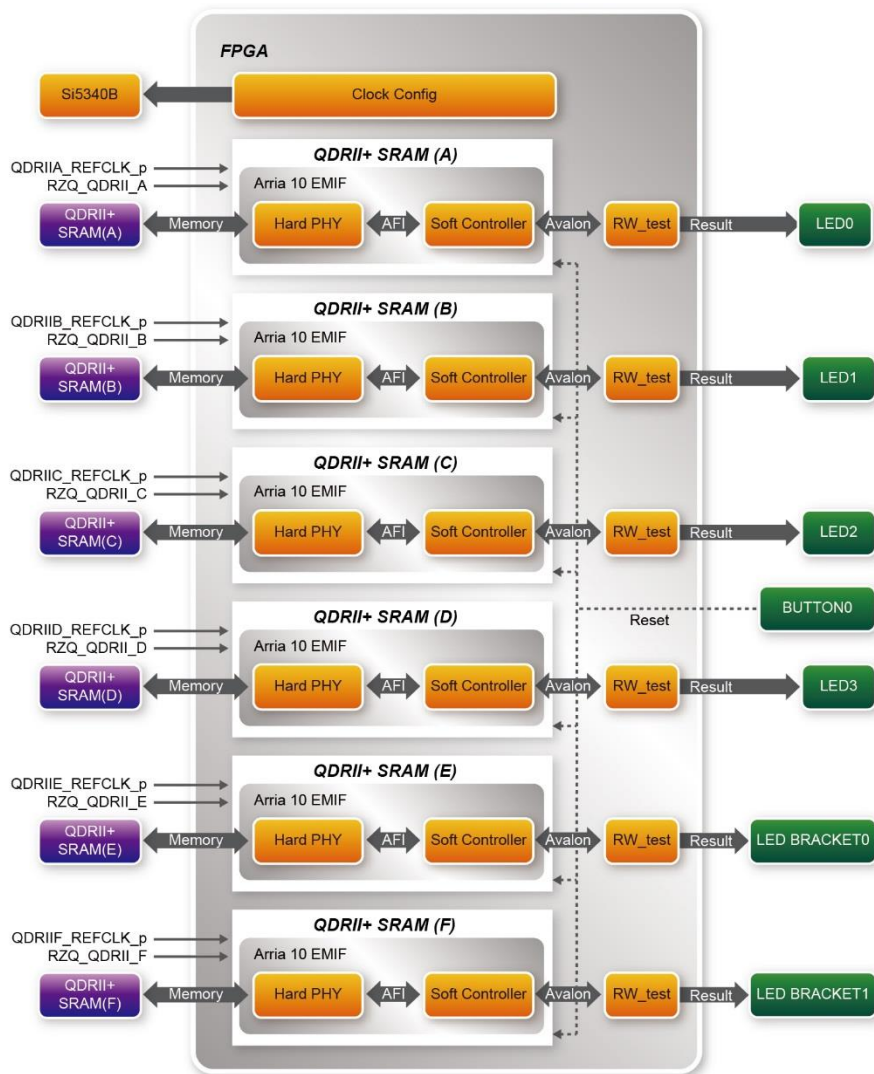
Figure 6-1 shows the function block diagram of the demonstration. The six QDRII+ SRAM controllers are configured as a 72Mb controller. The QDRII+ SRAM IP generates a 550MHz clock as memory clock and a half-rate system clock, 275MHz, for the controllers.
