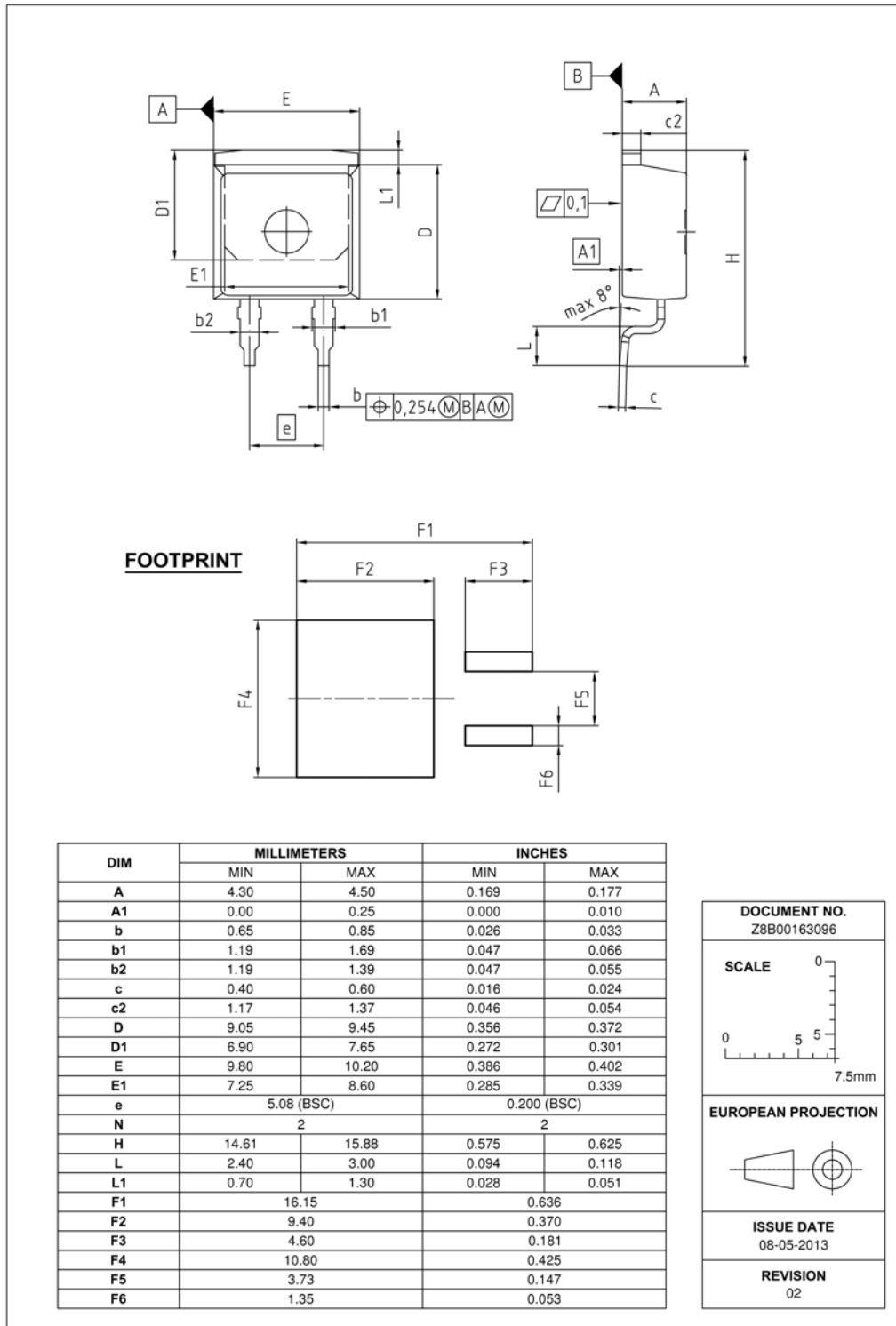
Figure 1 Outlines TO-263, dimensions in mm/inches
