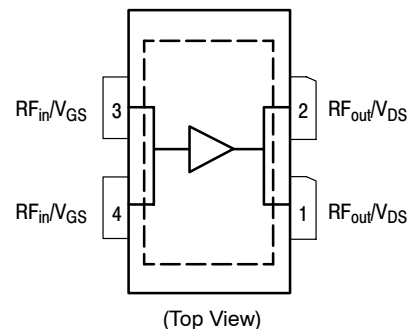
Figure 1. Pin Connections
