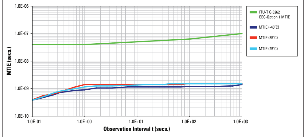
Wander Generation (MTIE) ITU-T G.8262 for EEC-Option 1
