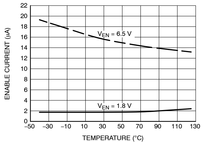
Figure 14. Enable Pin Input Current vs. Temperature
