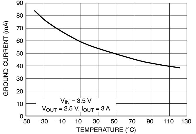
Figure 12. Ground Current vs. Temperature
