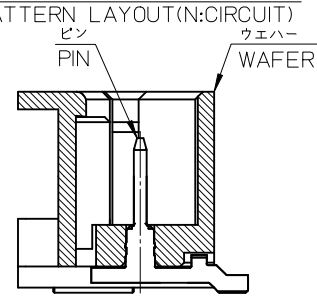
SECTION Z-Z
