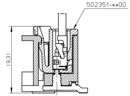
MATED DRAWING
