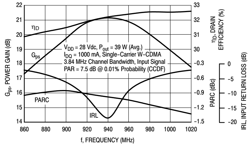
Figure 3. Single-Carrier W-CDMA Broadband Performance @ P out = 39 Watts Avg.
