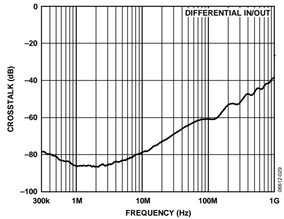
Figure 29. AD8105 Crosstalk, One Adjacent Channel
